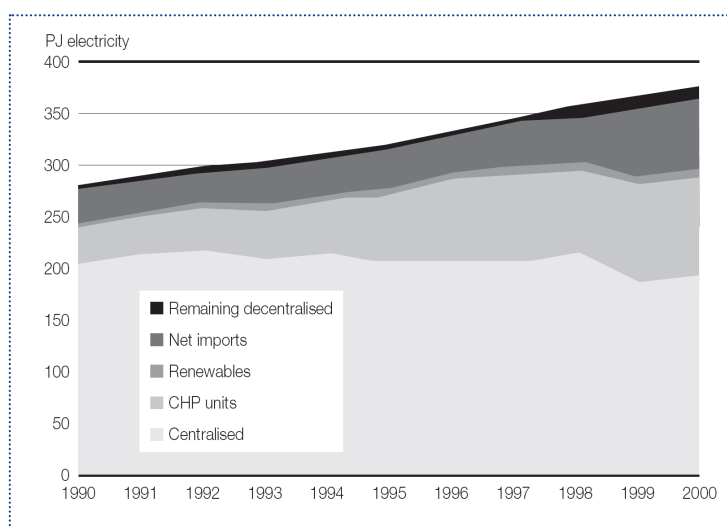
Figure 30c: Electricity production by source 1990-2000 (in PJ electricity)
