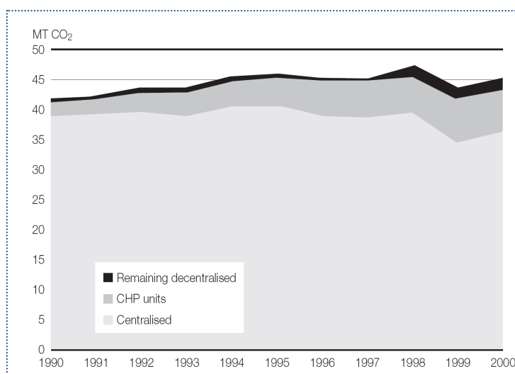
Figure 31: CO 2 emissions by energy source
